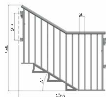
7058050 Handledare 1655x500 24,0 kg
